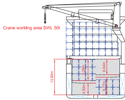
Hold No. 2 + 3
