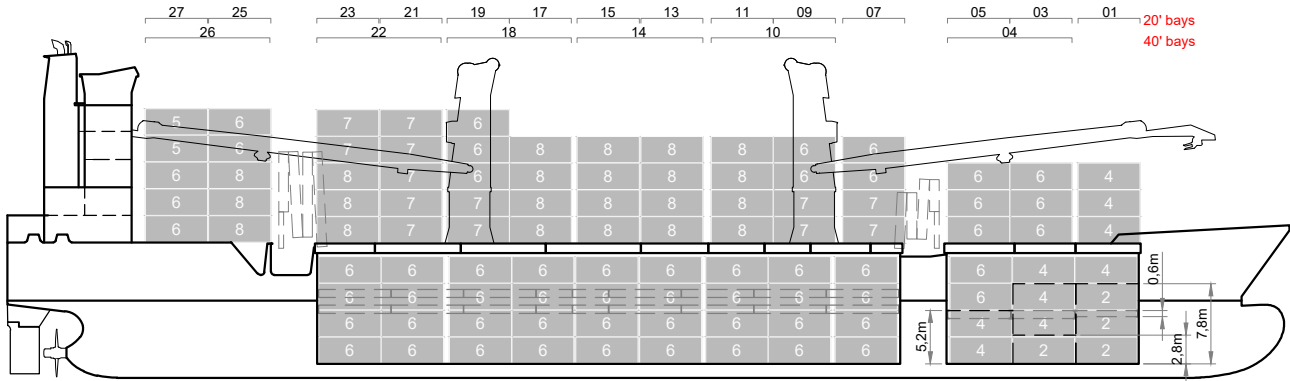
MAIN DECK
