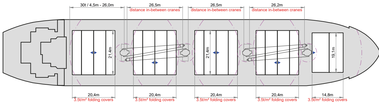
MAIN DECK
