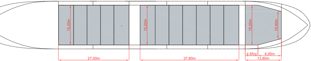
HOLDS & DOUBLE BOTTOM
