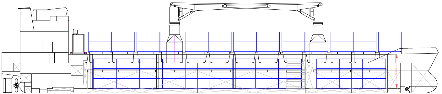
MAIN DECK
